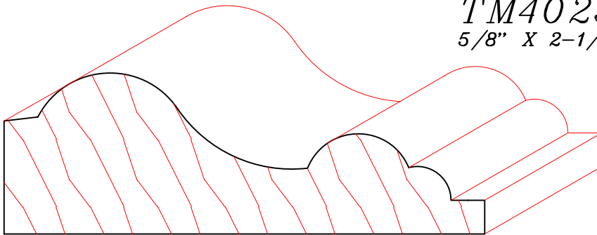
TM4024 1-3/16" X 3-9/16"
