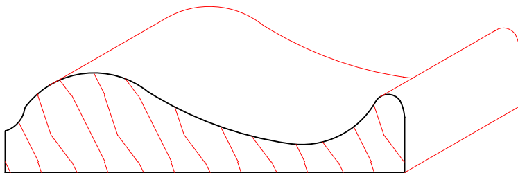
TM4046 3/4" X 3"
