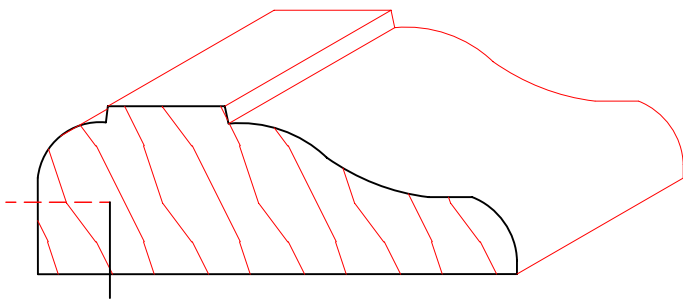
TM4031 7/8" X 2-1/2"
