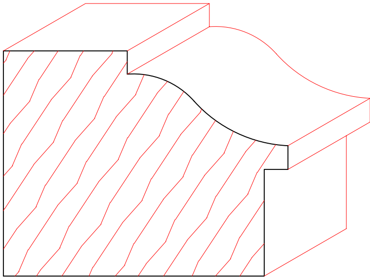
TM4034 2-3/8" X 3"
