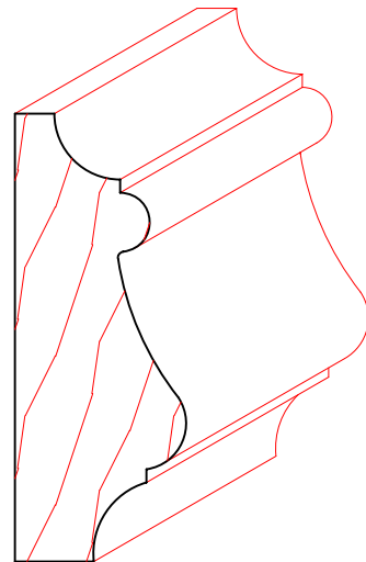
TM4005 13/16" X 2-1/8"
