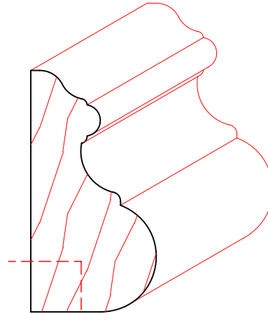
TM4007 7/8" X 1-3/4"
