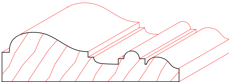
TM4040 13/16" X 3"
