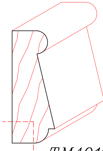
TM4017 3/4" X 2"
