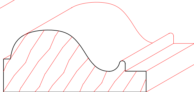
TM4041 1-1/8" X 2-9/16"
