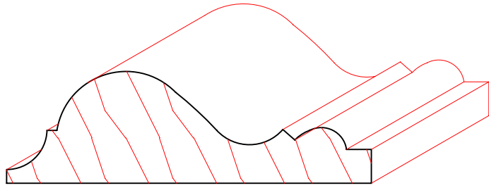
TM4027 13/16" X 2-11/16"
