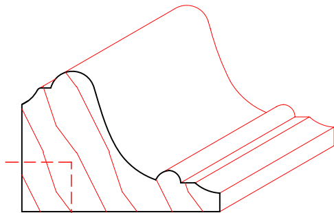
TM4010 1-1/16" X 1-1/2"
