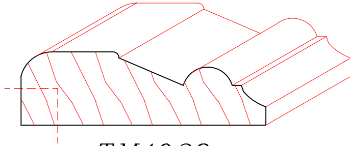
TM4028 3/4" X 2-1/2"
