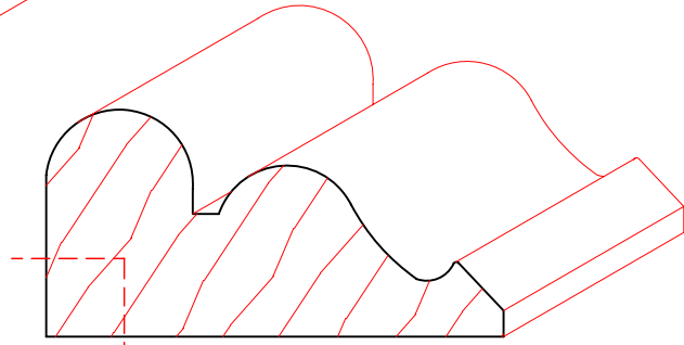
TM4030 1-1/16" X 2-3/16"
