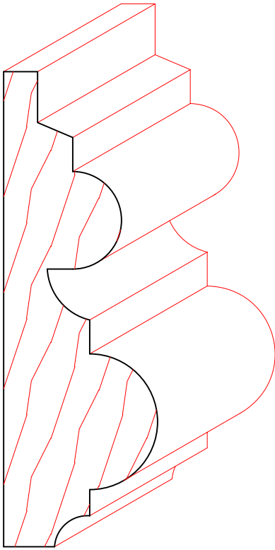
TM4001 1-1/16" X 3-5/8"
