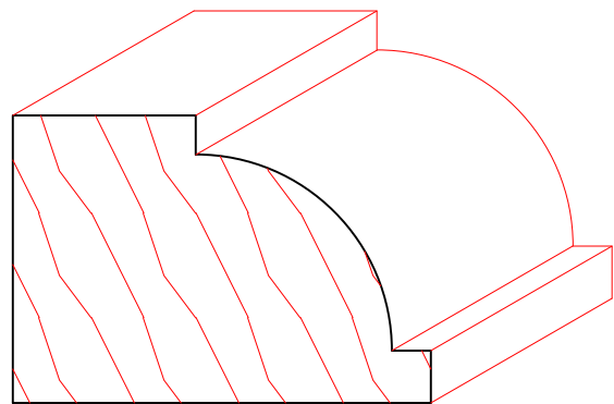
TM6009 1-3/8" X 2"
