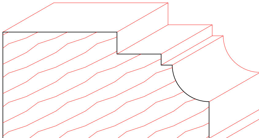
TM6016 1-3/4" X 3-1/2"
