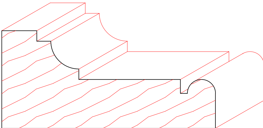
TM6014 1-3/4" X 3-7/8"
