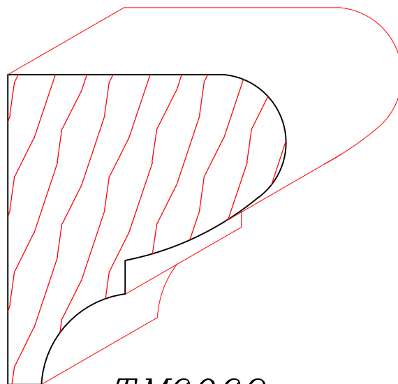
TM6069 2-1/16" X 2-5/16"
