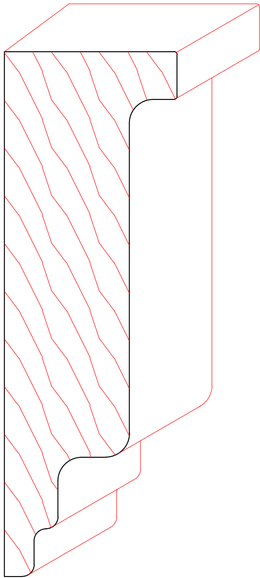
TM6052 1-13/16" x 5-1/2"
