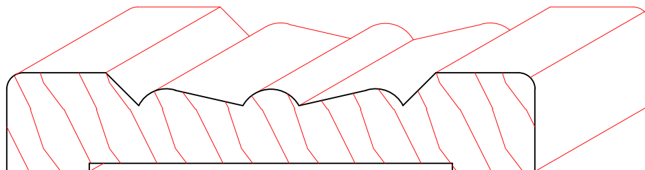
TM1097 3/4" X 4"
