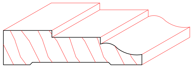
TM1012 5/8" X 2-1/2"
