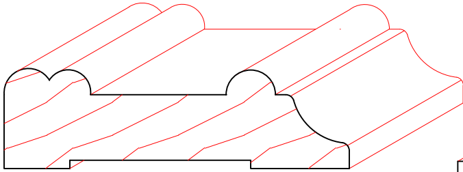
TM1072 3/4" X 2-5/8"
