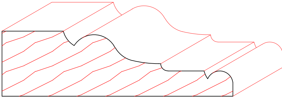
TM1231 1-1/8" X 4"
