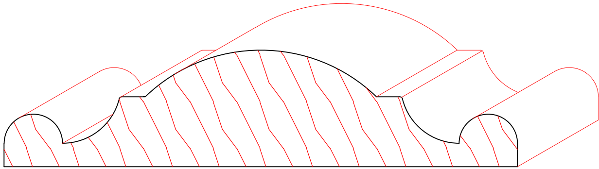
TM1230 1-1/4" X 5-1/2"
