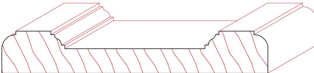
TM1249 3/4" X 4-3/4"
