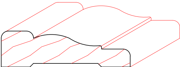
TM1005 5/8" X 2-1/4"
