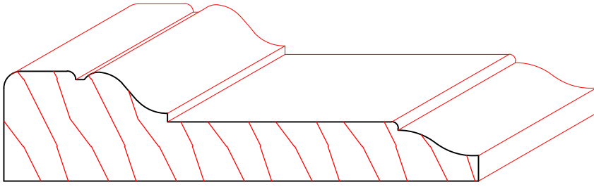
TM1225 13/16" X 3-1/2"
