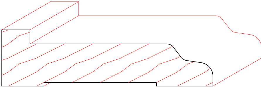
TM1134 1" x 3-3/4"
