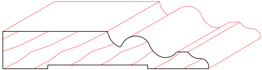
TM1040 5/8" X 3-7/16"
