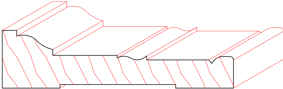
TM1068 1" X 4"
