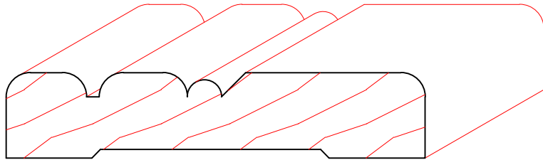
TM1022 5/8" X 3-1/16"
