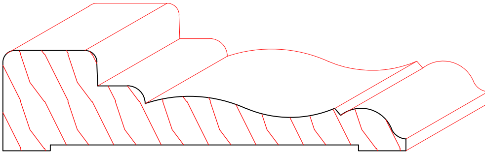
TM1187 1-1/16" X 4-1/4"
