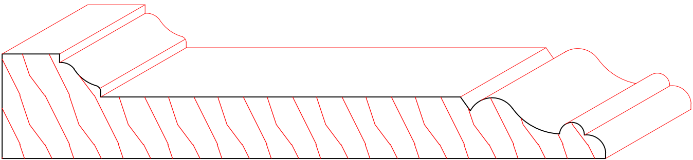
TM1212 1-1/16" X 7-1/4" (NOT TO SCALE)
