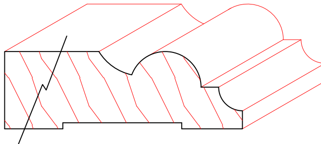
TM1018 13/16" X 2-1/2" +-
