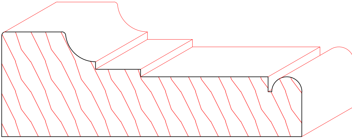
TM1247 1-3/4" X 5"
