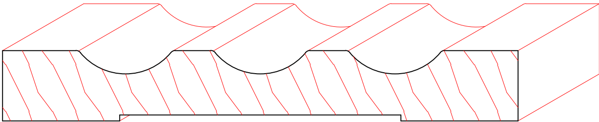
TM1076 3/4" X 5-1/2"
