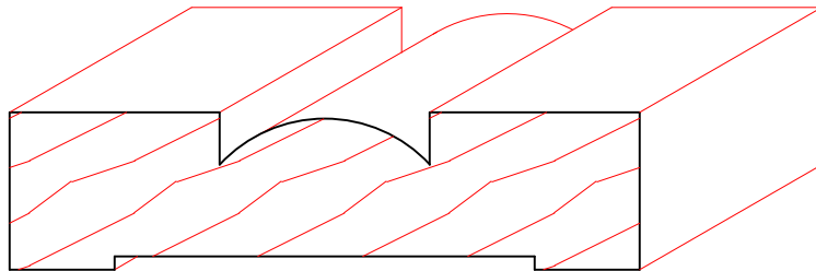
TM1126 3/4" X 3"
