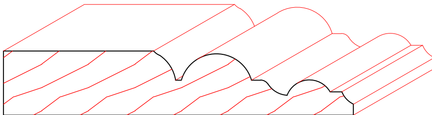
TM1202 11/16" X 3-3/4"
