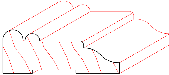
TM1138 3/4" X 2"
