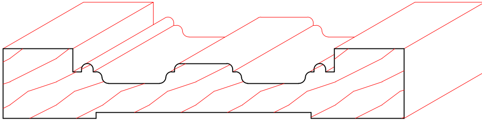
TM1061 3/4" x 4-5/16"
