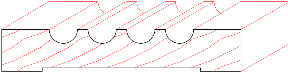
TM1055 3/4" x 4-1/4"
