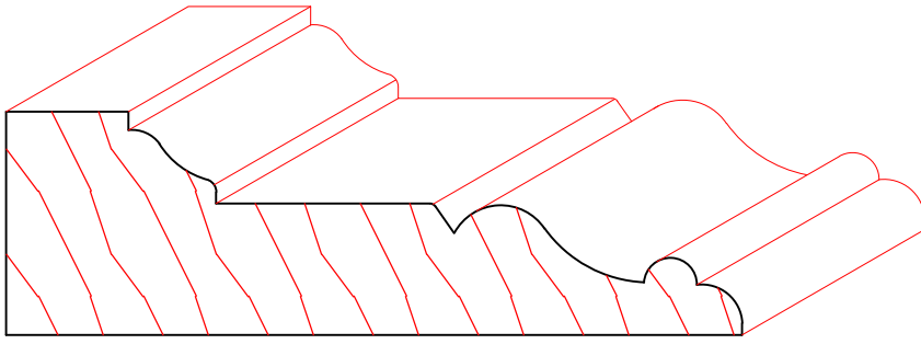
TM1212 1-1/16" X 3-1/2"
