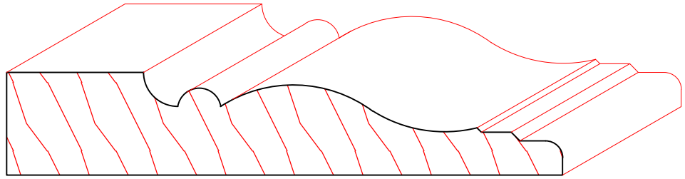
TM1239 3/4" X 4-1/16"
