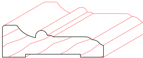
TM1093 3/4" X 2-3/16"
