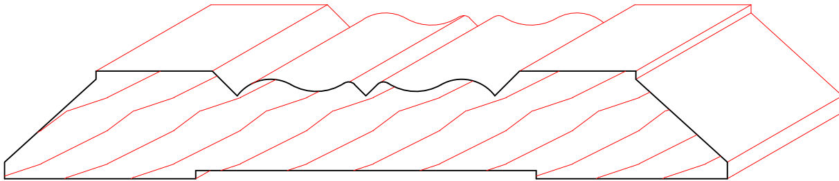
TM1151 13/16" X 5-7/16"
