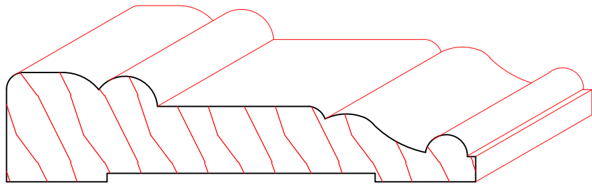
TM1194 13/16" X 3-1/2"
