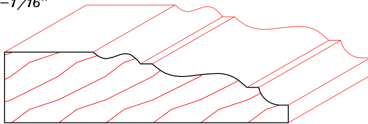
TM1236 3/4" X 3"
