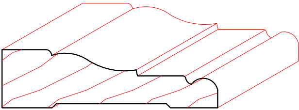
TM1001 5/8" X 2-5/16"
