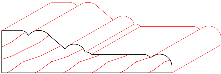
TM1200 3/4" X 3"
