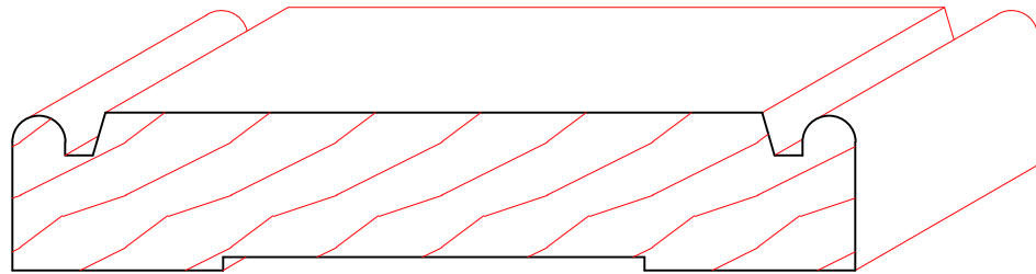
TM1069 3/4" X 4"
