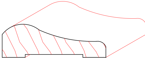
TM1070 3/4" X 2-1/4"
