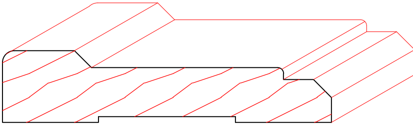
TM1193 3/4" X 3-7/16"
