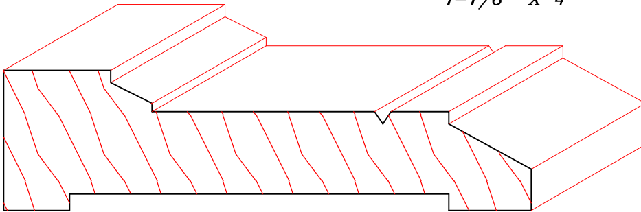
TM1188 1-1/6" X 4"
