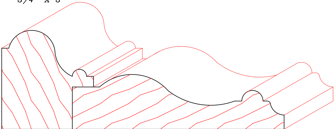
TM1201 1-3/4" X 5"
