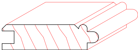
TM8039 9/16" X 2-1/8" +-
