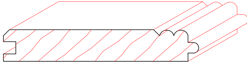
TM8017 9/16" X 3-1/2"
