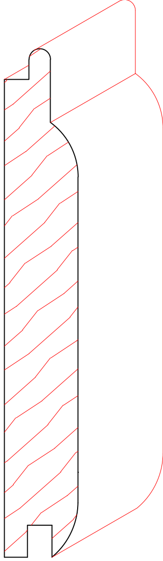
TM8021 3/4" X 5-1/4"
