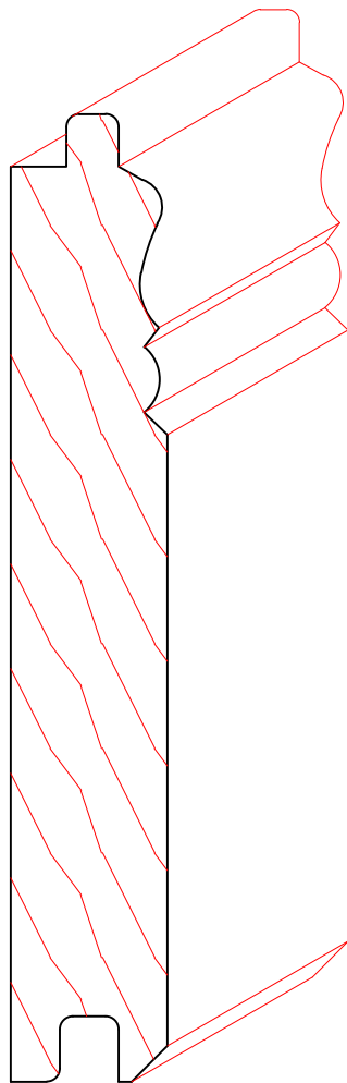
TM8023 3/4" X 4-5/8" +-
