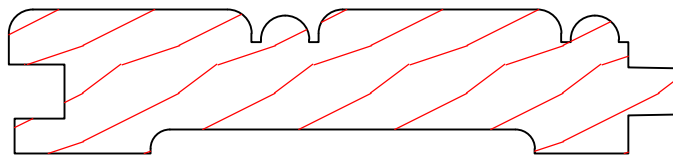
TM8040 3/4" X 3-1/2"
