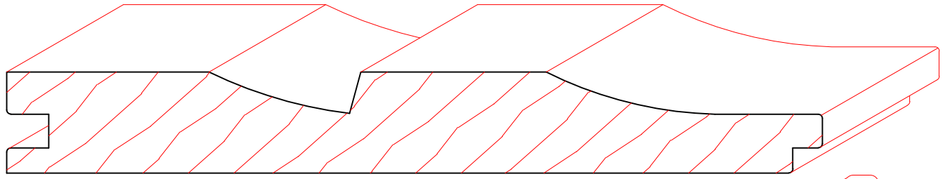
TM8028 3/4" X 6-1/16" +-
