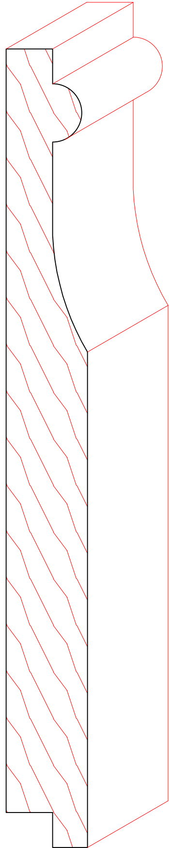
TM8048 7/8" X 8-9/16" +-
