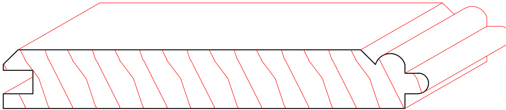
TM8016 5/8" X 4-1/2" +-
