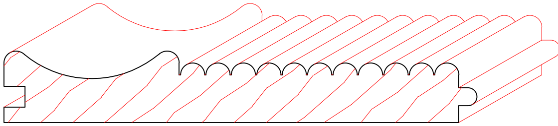
TM8018 3/4" X 5"
