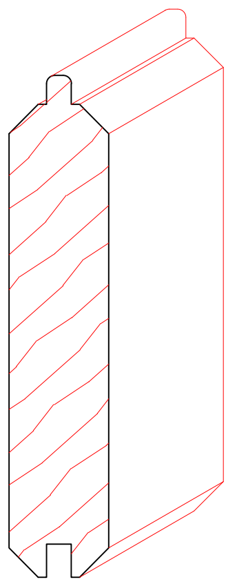
TM8025 3/4" X 3-3/16" +-
