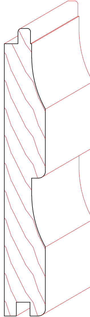
TM8007 3/4" X 5-3/16" +-
