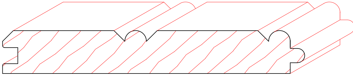
TM8042 13/16" X 3-1/4"
