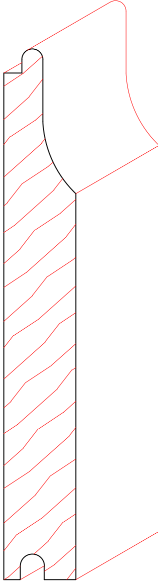
TM8006 3/4" X 5-1/2" +-
