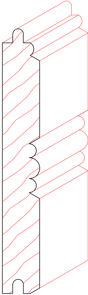
TM8004 11/16" X 4-3/4" +-
