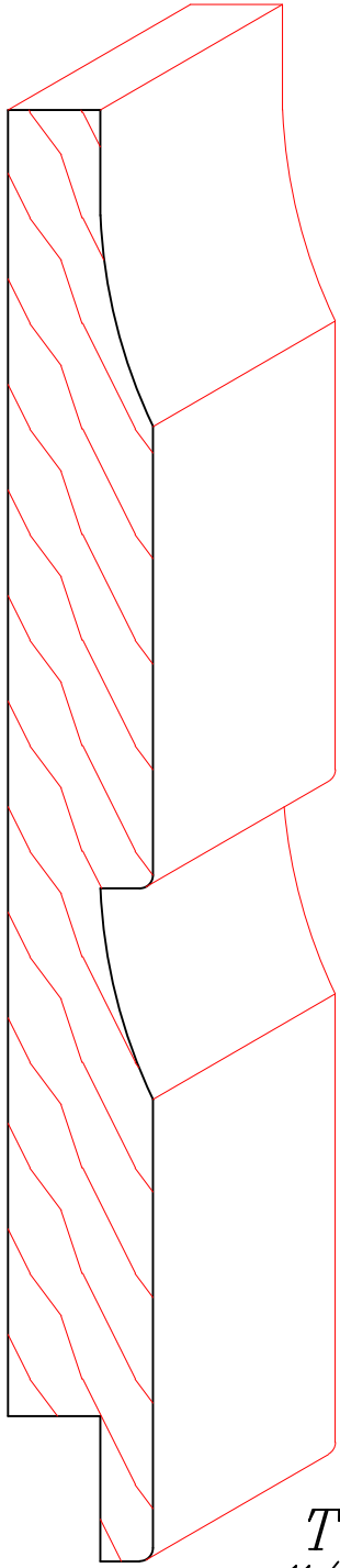
TM8027 3/4" X 3-1/2" +-
