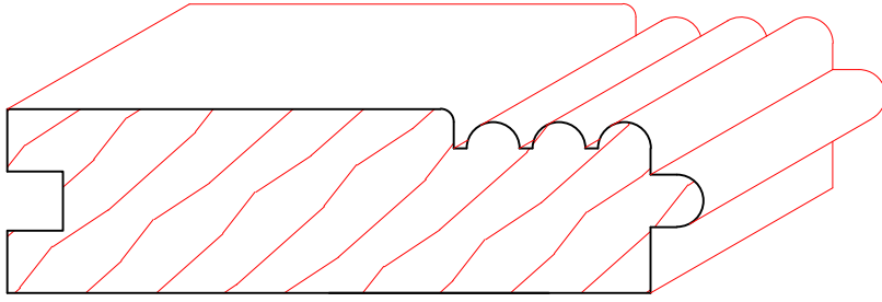
TM8045 7/8" X 3-5/16" +-
