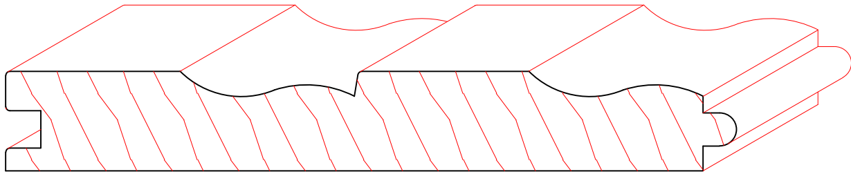
TM8011 3/4" X 5-1/2"
