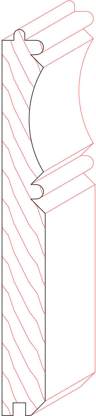
TM8019 3/4" X 6-5/8"
