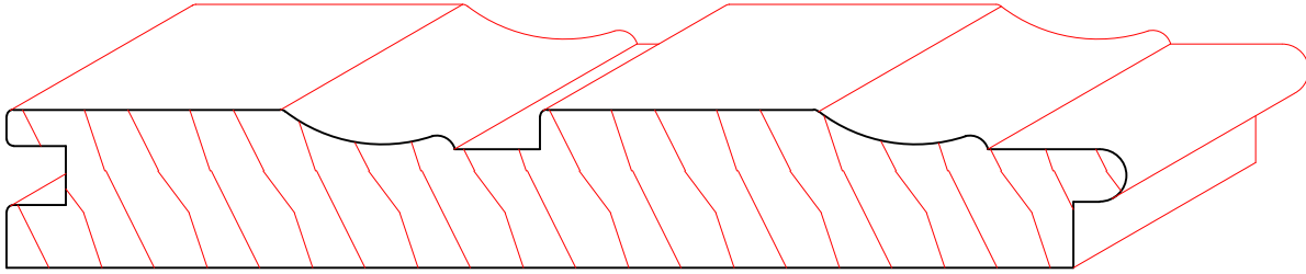
TM8014 3/4" X 5-5/16"
